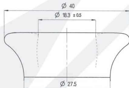
Finish detail
