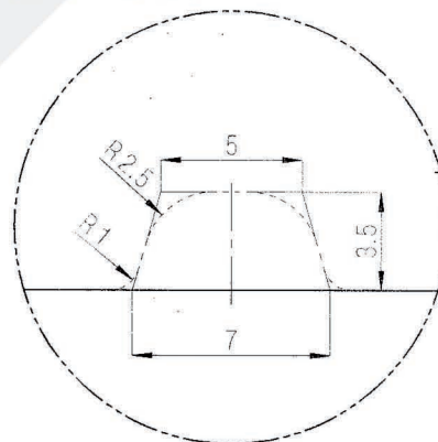
Detail A S 5:1
